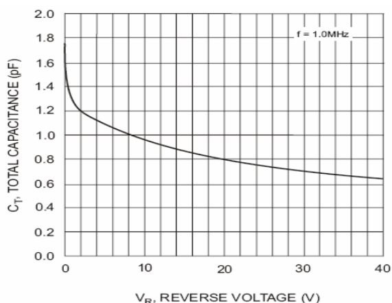
Fig. 3 Typical Capacitance vs. Reverse Voltage
